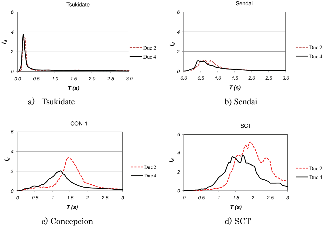
Fig. 3 Measure of seismic damage for 4 earthquake ground motion records
