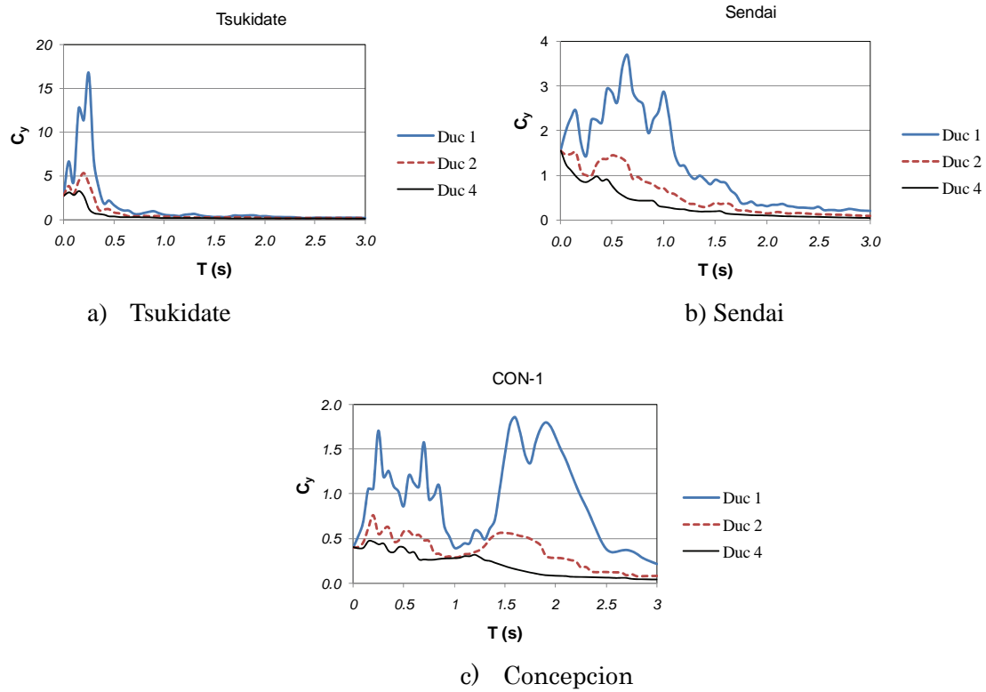
Fig. 2 C Y spectra for 3 earthquake ground motion records
