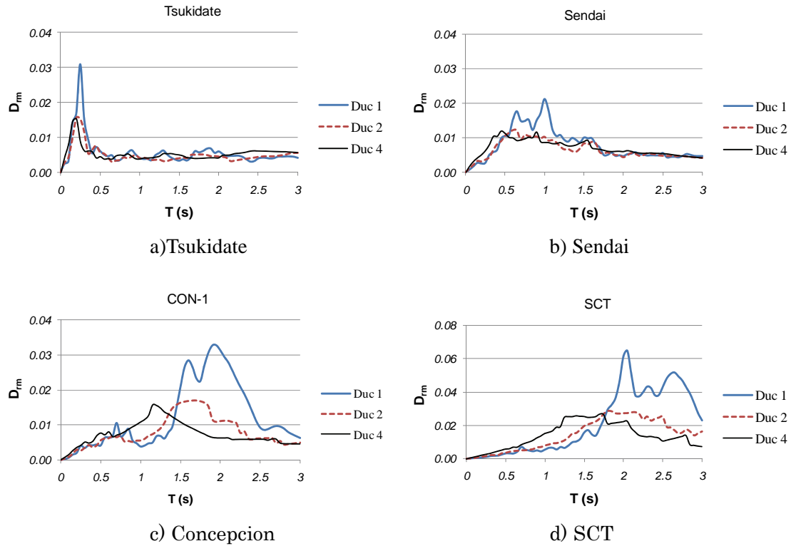
Fig. 1 D_m spectra for 4 earthquake ground motion records
