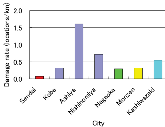
Fig. 3 Comparison of damage rate.
