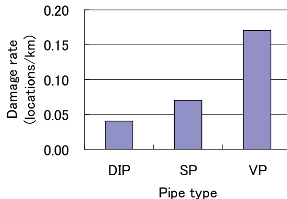
Fig. 1 Damage rate related to pipe type.
