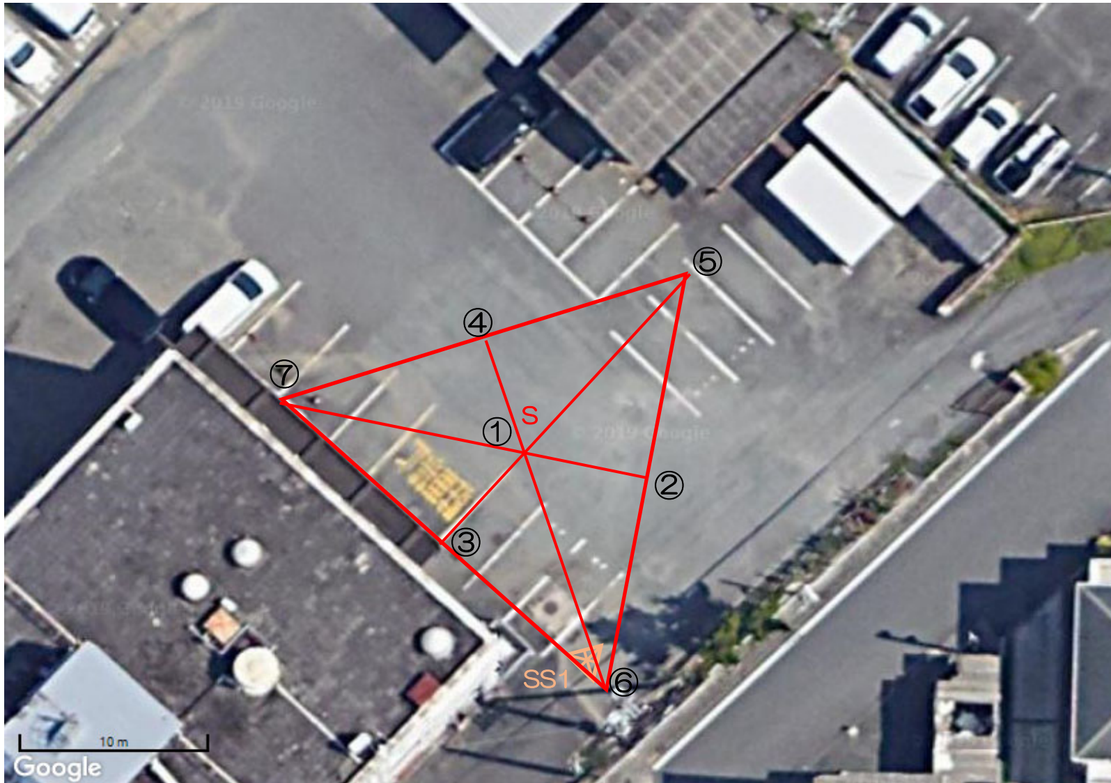
Array configuration for KUM-SS1 (1m-2m) and KUM-S (10m-20m)
