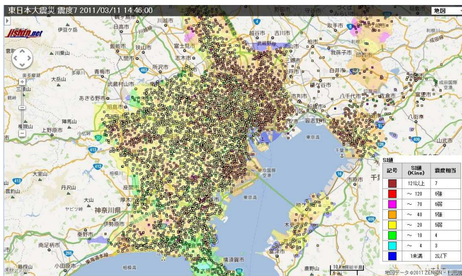
Fig.3 SI values observed by SI Sensors and Interpolated SI Values by 50m Meshes
