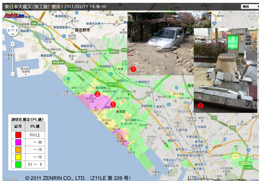
Fig.4 Estimation of Risk of Liquefaction by SUPREME and Actual Liquefaction Damage
