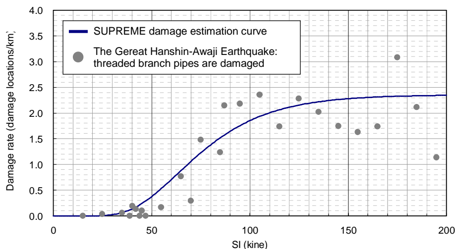
Fig.2 Damage Estimation Curve of SUPREME
