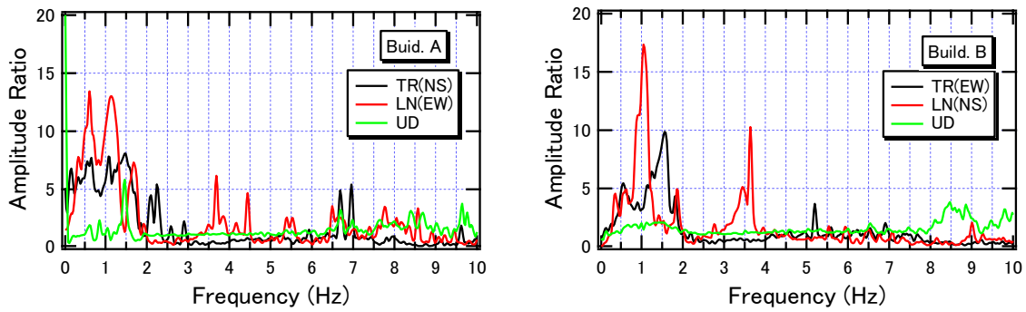
Fig. 12 Amplitude ratios between 14F/1F of the building A and B
