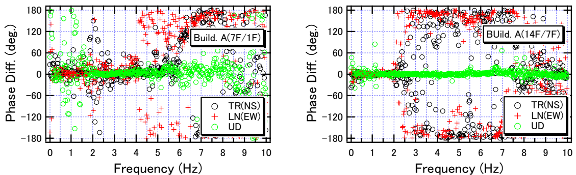
Fig. 9 Phase differences between 7F /1F and 14F/7F of the building A
