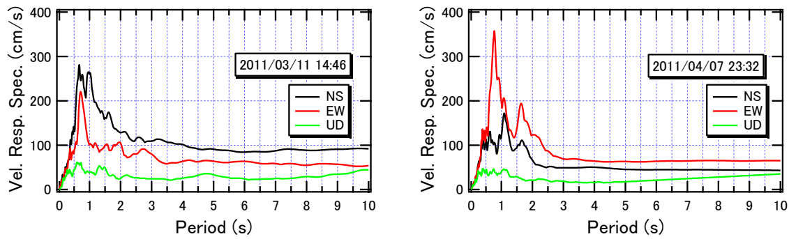
Fig. 2 Velocity response spectra ( h=5\% ) at MYG013 Left: 2011/03/11 main shock, Right: 2011/04/07 aftershock
