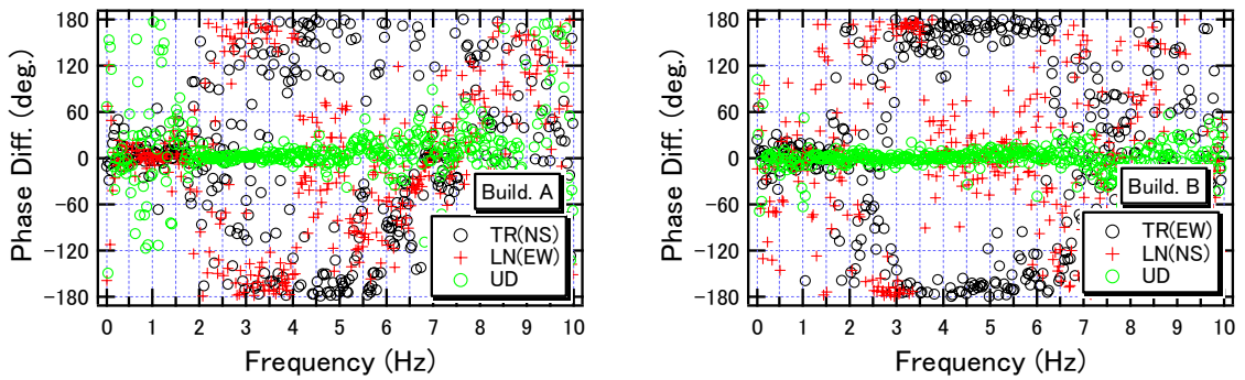
Fig. 13 Phase differences between 14F/1F of the building A and B
