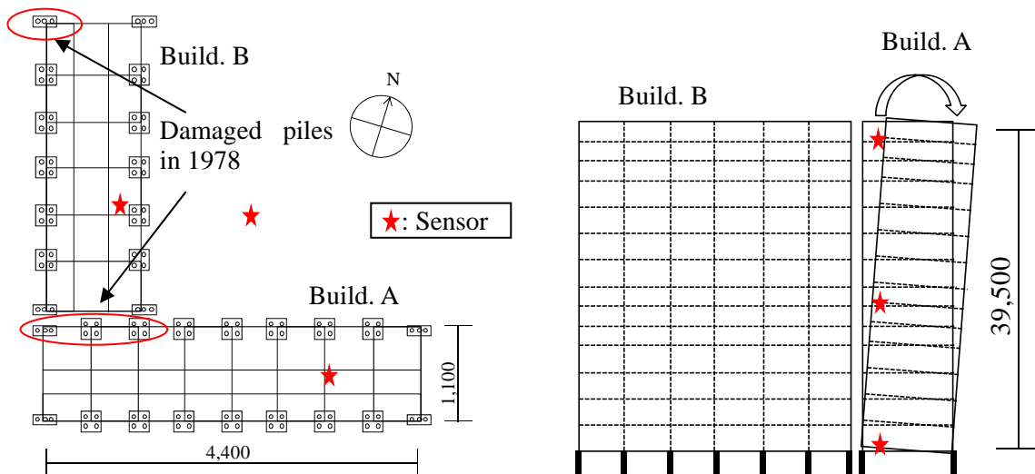
Fig. 6 Schematic plan and façade of the housing complex of STM
