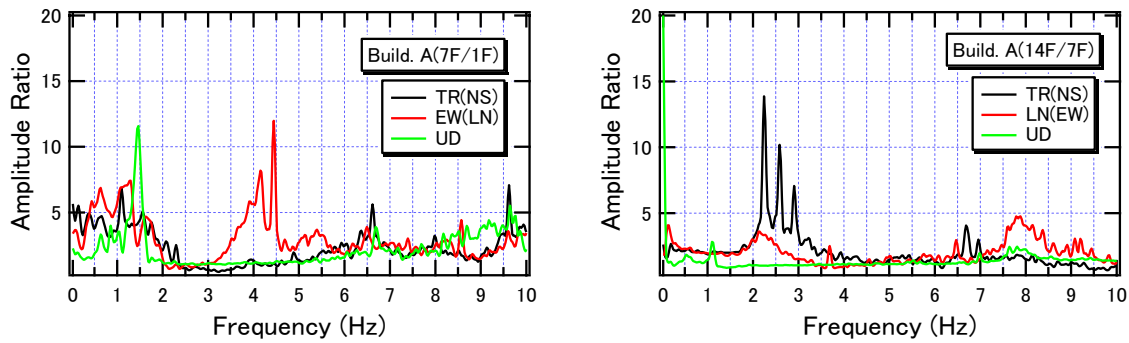
Fig. 8 Amplitude ratios between 7F /1F and 14F/7F of the building A
