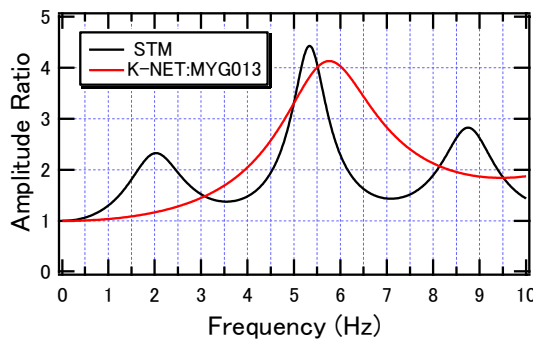
Fig. 5 Theoretical amplitude characteristics of the site of STM and MYG013 (K-NET)
