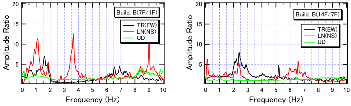
Fig. 10 Amplitude ratios between 7F /1F and 14F/7F of the building B
