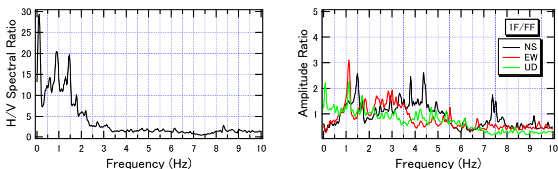
Fig. 14 H/V spectrum of the ground and amplitude ratios between 1F and the free field
