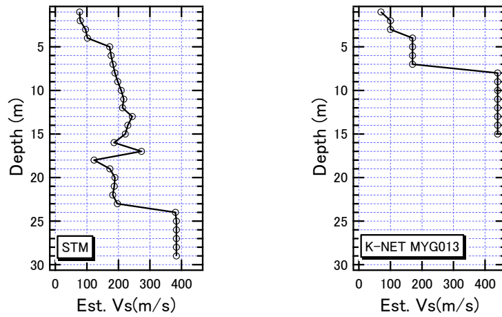
Fig. 4 Estimated Shear wave velocity distribution of the site of STM and MYG013 (K-NET)
