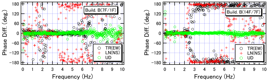
Fig. 11 Phase differences between 7F /1F and 14F/7F of the building B
