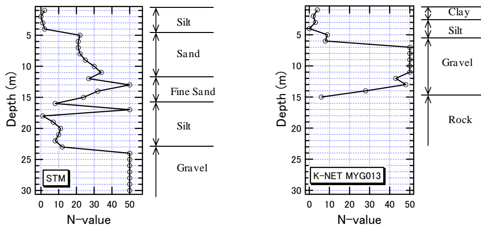
Fig. 3 N-value distribution of the site of STM and MYG013 (K-NET)
