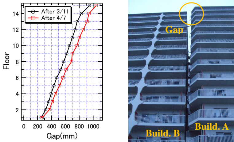
Fig. 7 Measured gap between the building A and B
